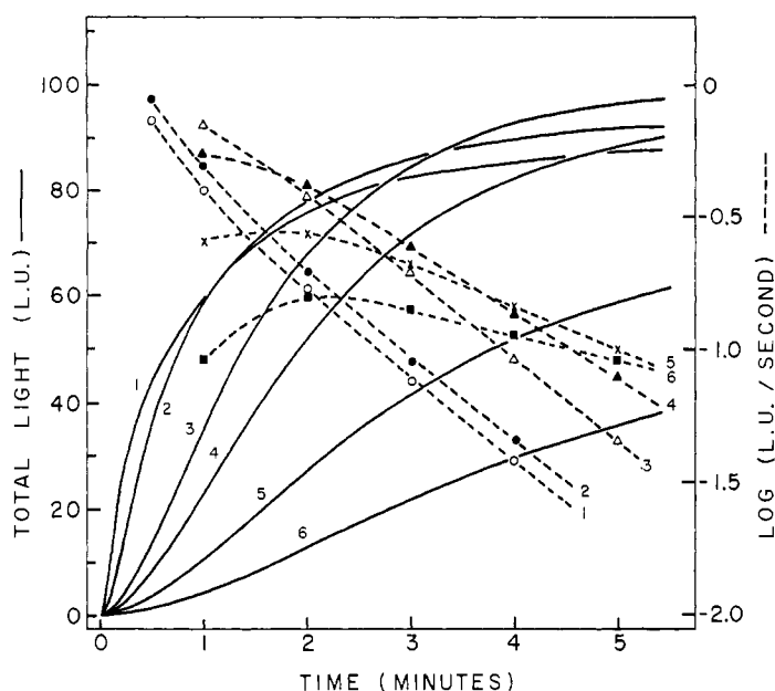
FIGURE 6: Influence of purple protein concentration on total light produced and intensity of luminescence as a function of time, with constant initial concentrations of luciferin and luciferase. Reaction mixtures in 5 ml of buffer contained 10\ \mu\text{l} of luciferase of optical density = 1.2/\text{cm} at 280\ \text{m}\mu , 10\ \mu\text{l} of luciferin solution, and the following amounts of purple protein of optical density = 0.6/\text{cm} at 280\ \text{m}\mu : curve 1, 20\ \mu\text{l} ; curve 2, 5\ \mu\text{l} ; curve 3, 1\ \mu\text{l} ; curve 4, 0.5\ \mu\text{l} ; curve 5, 0.2\ \mu\text{l} ; and curve 6, none added.
