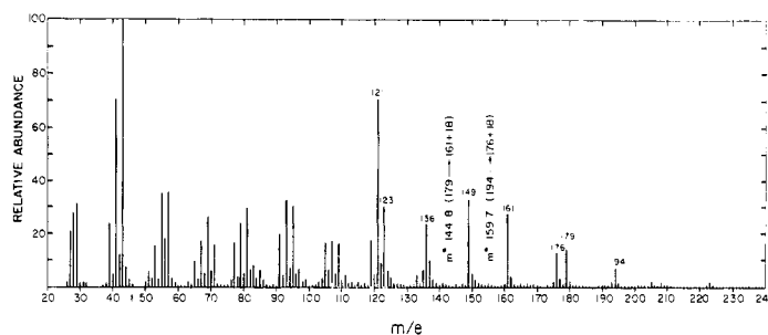
FIGURE 8: Mass spectrum of the product of luciferin in the bioluminescence reaction, 70 eV. The water used in the reaction was found to contain traces of impurities which give an intense peak at m/e 149 and also several peaks in the low m/e region with the highest at m/e 57.
