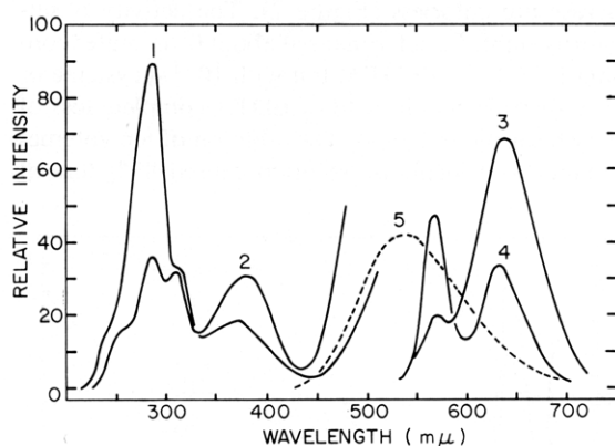
FIGURE 4: Fluorescence spectra of purple protein solution, optical density 0.45/cm at 280 m\mu (solid line), and bioluminescence spectrum of the purified system (broken line), measured on an Aminco-Bowman spectrophotofluorometer with the corrected spectra attachment. (1) Excitation spectrum recorded at 630 m\mu ; (2) excitation spectrum recorded at 565 m\mu ; (3) emission spectrum excited at 285 m\mu ; (4) emission spectrum excited at 380 m\mu ; and (5) bioluminescence spectrum of a reaction mixture of 10,000 LU of luciferin, 1 \mu l of purple protein (optical density 0.45/cm at 280 m\mu ) and 10 \mu l of luciferase solution (optical density 2.7/cm at 280 m\mu ) in 5 ml of buffer.
