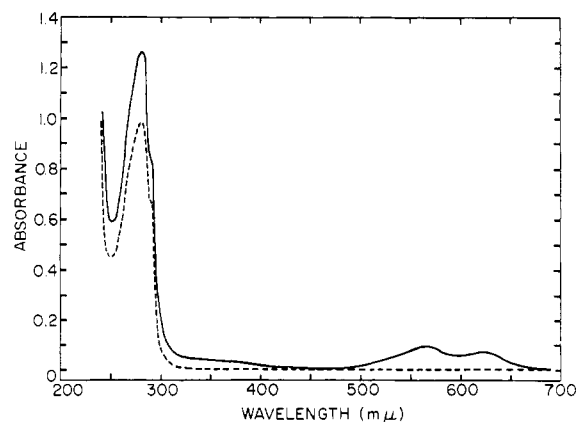
FIGURE 2: Absorption spectra of luciferase (broken line) and purple protein (solid line), measured on a Perkin-Elmer 202 spectrophotometer.
