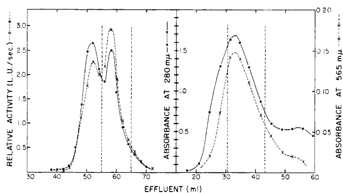
FIGURE 1: Elution curves. Left: of luciferase from the final DEAE-cellulose column. Right: of purple protein from the final Bio-Gel P-100 column. Since activity of the purple protein is not proportional to concentration, absorbance at 565 \text{ m}\mu is plotted instead of activity.
