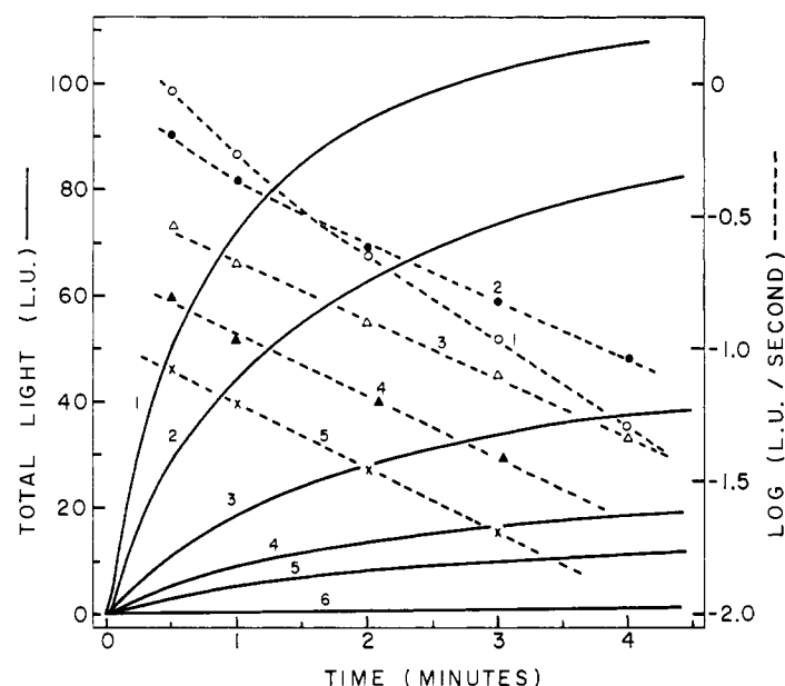
FIGURE 5: Influence of luciferase concentration on total light produced and intensity of luminescence as a function of time, with constant initial concentrations of luciferin and purple protein. Reaction mixtures in 5 ml of buffer contained 10 \mu l of luciferin solution, 10 \mu l of purple protein solution of optical density = 0.6/cm at 280 m \mu , and luciferase solution of optical density = 1.2/cm at 280 m \mu in the following amounts: curve 1, 10 \mu l; curve 2, 5 \mu l; curve 3, 2 \mu l; curve 4, 1 \mu l; curve 5, 0.5 \mu l; and curve 6, none added. The just detectable light produced in the absence of added luciferase is most probably attributable to a trace of luciferase contaminating the purple protein solution.
