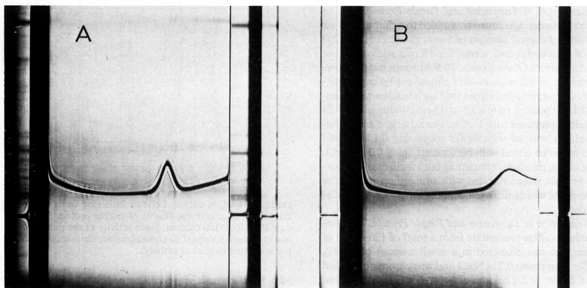
FIGURE 3: Ultracentrifugal pattern of luciferase at 2.8^\circ (left) and of purple protein at 3.4^\circ (right), both at 59,780 rpm, in 0.015 M sodium phosphate-0.00025 M EDTA-0.1 M NaCl (pH 6.8) (after 56 min).
