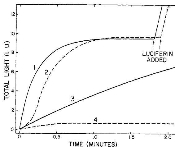
FIGURE 7: Influence of 2 \times 10^{-4}\ \text{M}\ \text{Fe}^{2+} as \text{Fe}(\text{NH}_4)_2(\text{SO}_4)_2 on the time course and total light produced after incubating for 2 min with different combinations of reactants as follows: curve 1, (purple protein + luciferase + \text{Fe}^{2+} ) + (luciferin), or (purple protein + \text{Fe}^{2+} ) + (luciferase + luciferin); curve 2, (luciferase + \text{Fe}^{2+} ) + (purple protein + luciferin); curve 3, (luciferase) + (purple protein + luciferin) and curve 4, (purple protein + luciferin + \text{Fe}^{2+} ) + (luciferase). In each mixture, the amount of luciferase was sufficiently large for a fast reaction, and the amount of purple protein was small compared with that of luciferin.
